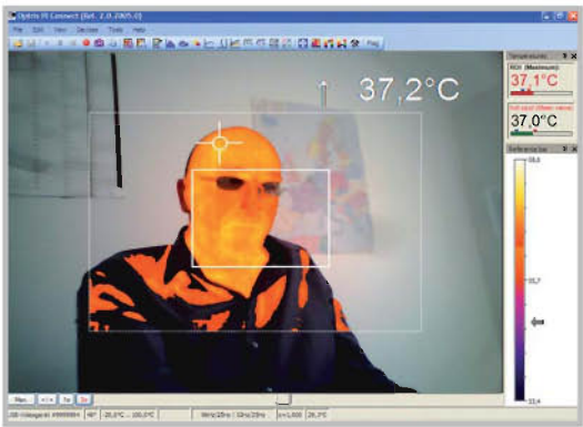
Cross-fading of VIS image above temperatures of 35°C
